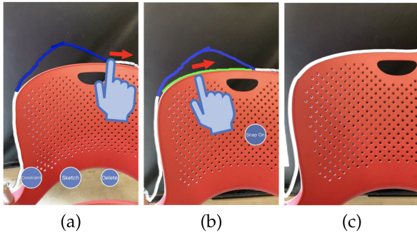
Fig. 13. 2D sketching. The user selects a curve segment (in blue in (a)), and draws a desired 2D curve (in green in (b)) in a frozen view. Edge snapping is used in (b) to help create accurate curves. The blue hand icon and the red arrow are added to the figure to illustrate the gesture interaction.
