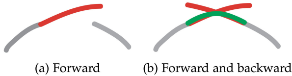
Fig. 9. A curve segment (in red) due to short-term track loss can be estimated between adjacent curve segments (in gray) based on the acceleration data from IMU. A fused curve (in green) from both forward and backward integration of acceleration reduces accumulation errors and better connects the curve segments in gray than using forward integration alone.
