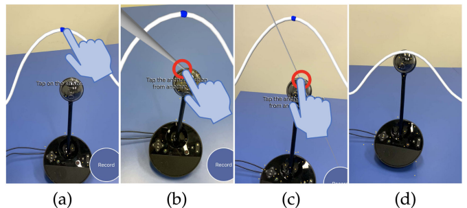
Fig. 12. Point constraint. (a) The user creates a curve around a rounded camera, but it is deviated from the top of the camera. To make the curve go through the top of the camera, the user first taps to select a point on the curve (blue point) to change. (b)(c) Then the user uses two-ray intersection to locate a target point (red circle) in two views. (d) The blue point will move to the target point and the whole curve is optimized to go through the target point. The blue hand icon and the red circle are added to the figure to illustrate the gesture interaction.
