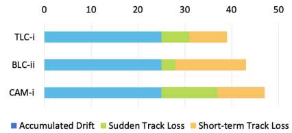
Fig. 7. Frequency of local tracking errors for each pair of input point and phone grip.
