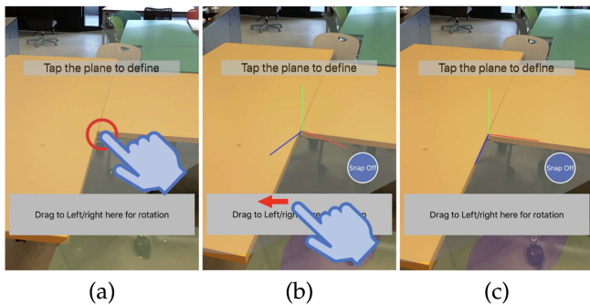
Fig. 11. World anchor re-localization. (a) Our system detects planes (semi-transparent gray planes in the figure). The user taps on a plane (red circle) to locate the origin of the world coordinate system. (b) In this example, the origin of the world coordinate system is located at the corner of the table. The user swipes left or right to change the world system's orientation. (c) The world coordinate system is located accurately with the desired orientation at the corner of the table. Edge snapping is used in (a) to help locate along physical edges in the image. The blue hand icon, the red arrow, and the red circle are added to the figure to illustrate the gesture interaction.
