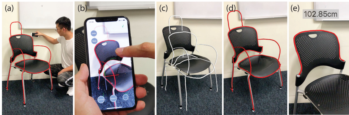
Fig. 1. We present a system for novice users to facilitate 3D curve creation on and around physical objects using an AR-enabled mobile device as a 3D pen (a), followed by interactive correction of curves with tracking errors (b). (c) and (d) show the results after initial creation (using 0.7 mins) and after interactive correction (using 5.6 mins), respectively. We also demonstrate our system with a 3D measurement application (e). The ground truth length is 106.1 cm for this example.
